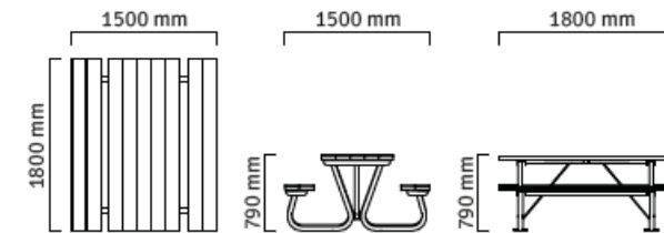
PICKNICK-GARNITUR
